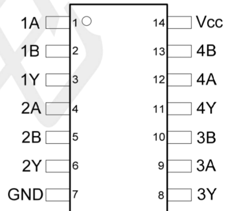
SOP-14
