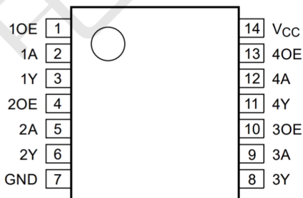
TSSOP-14
