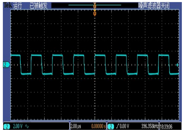
SW Noise ( V_{IN}=3.6V , I_{LOAD}=100mA )
