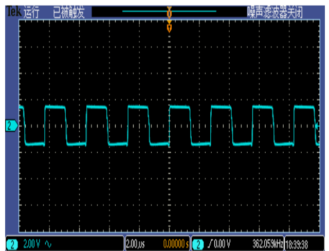
SW Noise ( V_{IN}=4.2V , I_{LOAD}=100mA )
