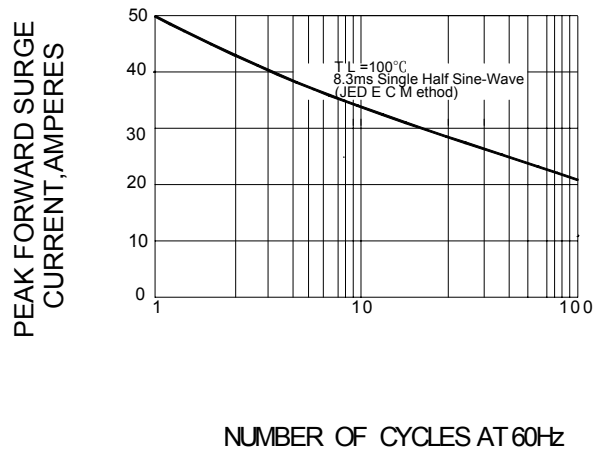
FIG.1- PEAK FORWARD SURGE CURRENT
