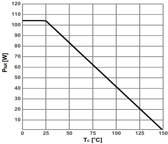
Figure 4: Power dissipation For TO-220、TO-252、TO-263
