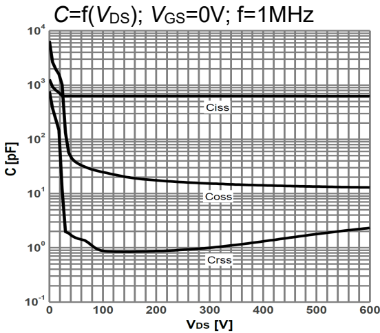
Figure 15: Typ. capacitances
