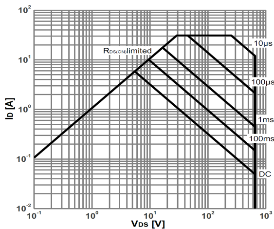
Figure 6: Safe operating area For TO-220F
