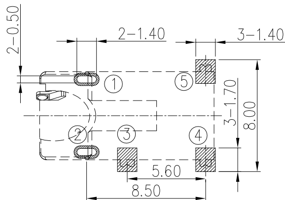
RECOMMENDED PCB LAYOUT (TOP VIEW) GENERAL TOLERANCES: ±0.05
