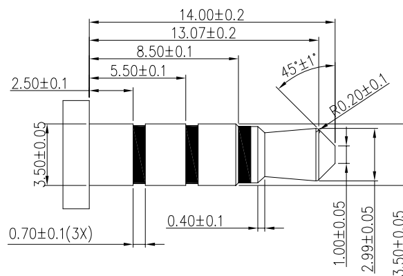
MALE PLUG SCHEMATIC
