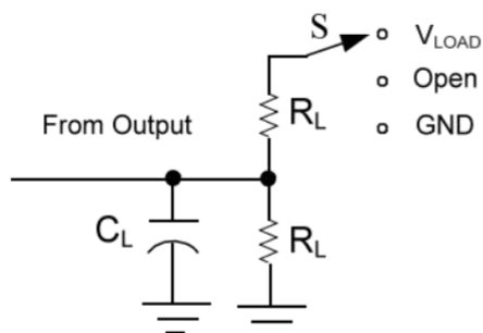
TEST CIRCUIT
