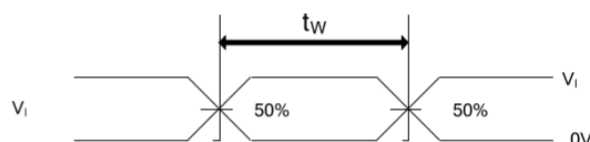
PULSE WIDTH
