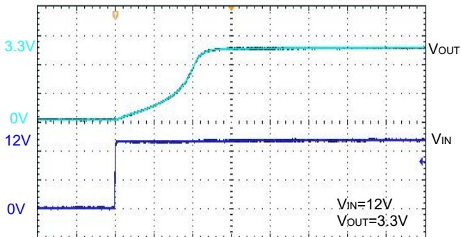
No-load start
