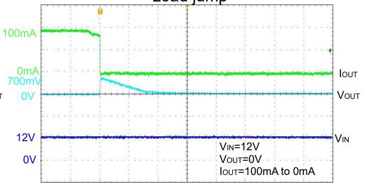
Load jump
