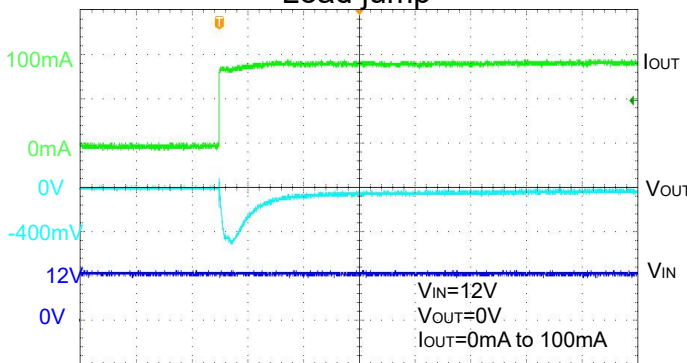
Load jump
