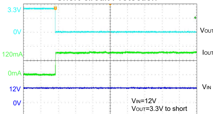
Short-circuit Protection
