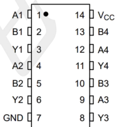
SOP-14
