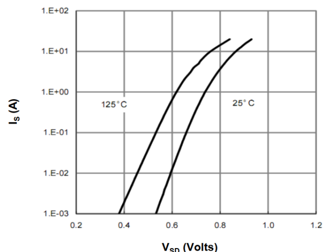
Figure 6: Body-Diode Characteristics
