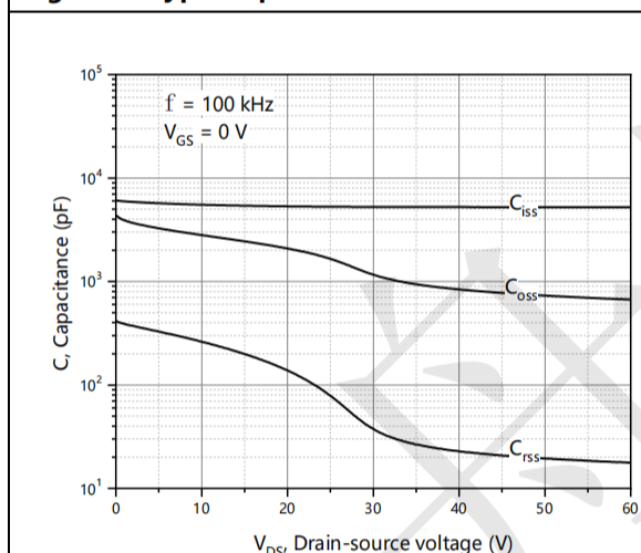
Figure 3. Typ. capacitances
