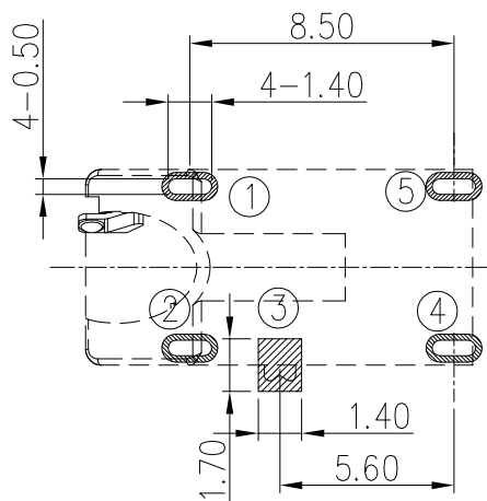
RECOMMENDED PCB LAYOUT (TOP VIEW) GENERAL TOLERANCES: \pm 0.05
