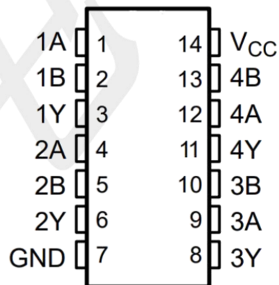
SOP-14
