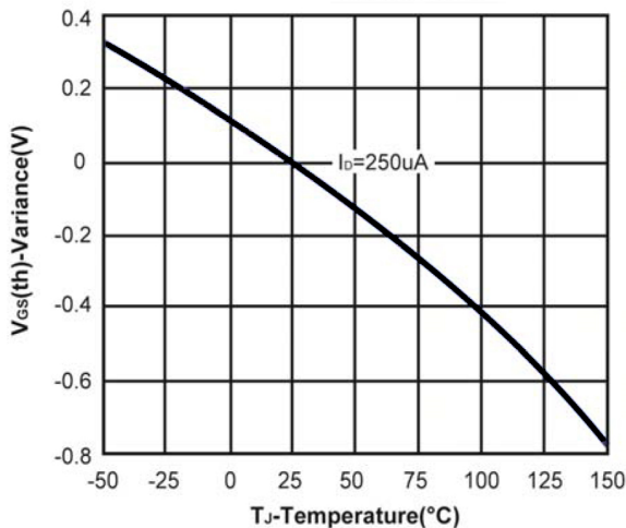
Figure 5 Threshold Voltage
