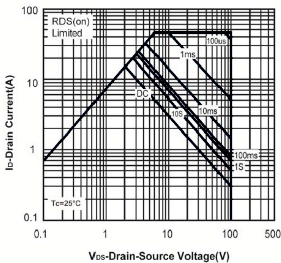
Figure 10 Maximum Forward Biased Safe Operating Area
