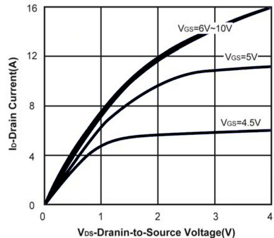
Figure 6 On-Region Characteristics
