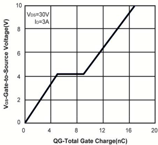
Figure 8 Gate Charge
