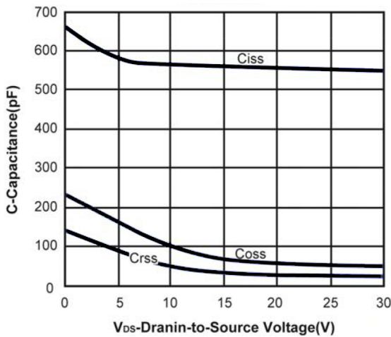
Figure 3 Capacitance
