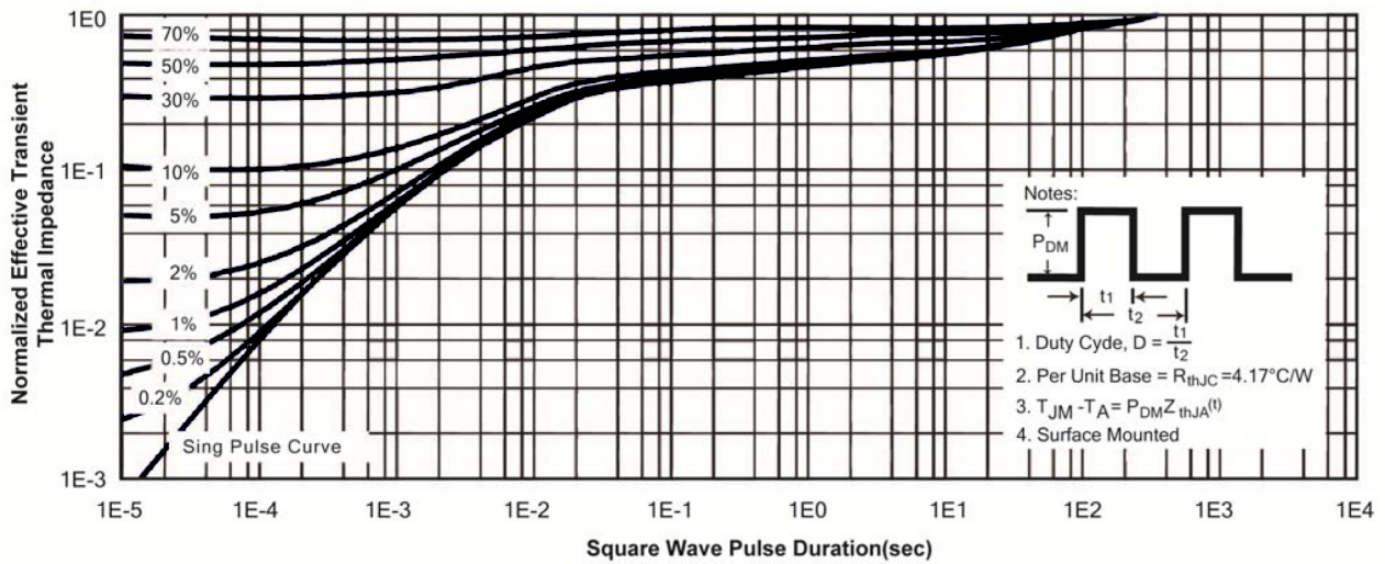
Figure 7 Normalized Thermal Transient Impedance, Junction-to-Case
