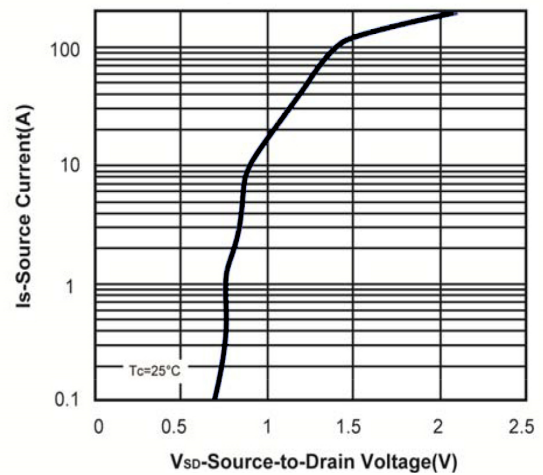
Figure 9 Body-diode characteristics
