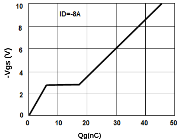
Figure8. Gate Charge Waveforms
