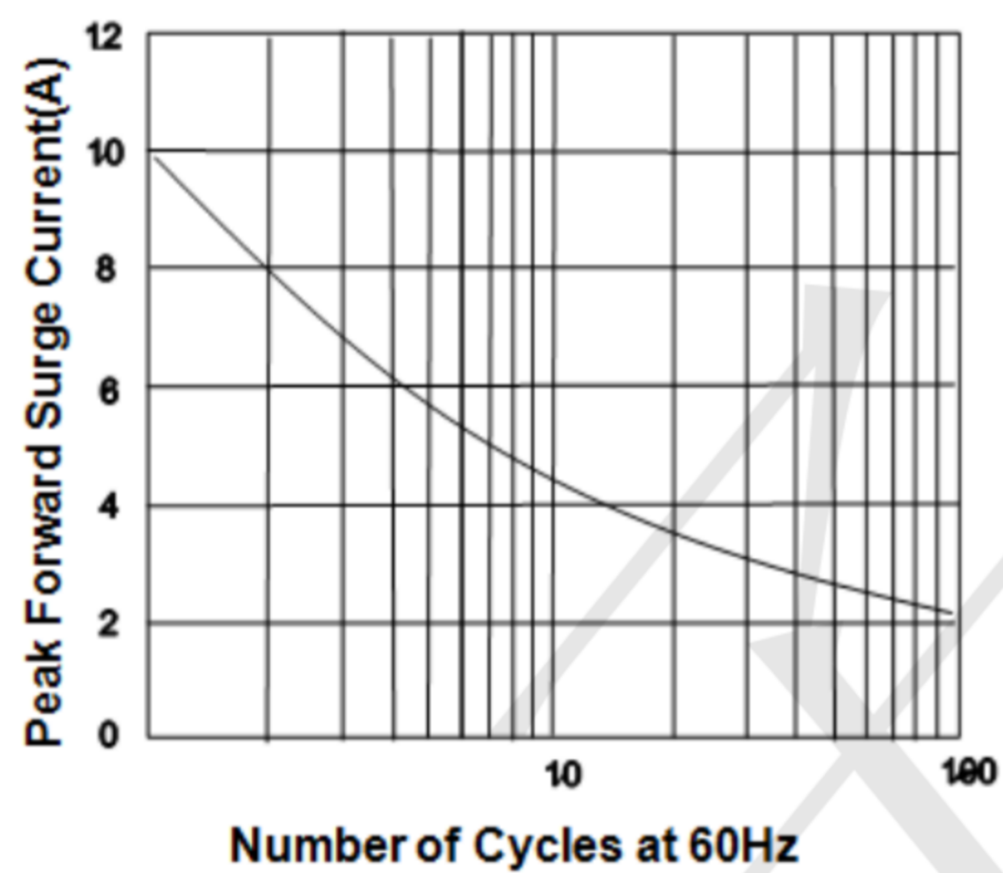
Fig.2 Maximum Non-Repetitive Peak Forward Surge Current
