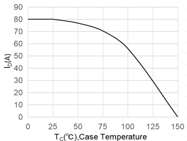
Figure 2: Current De-rating
