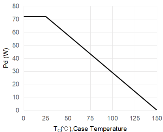
Figure 1: Power De-rating
