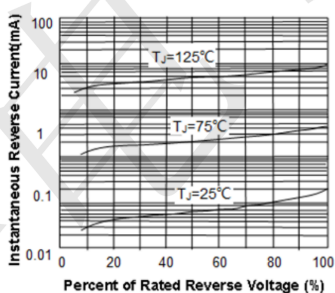
Fig.4 Typical Reverse Characteristics
