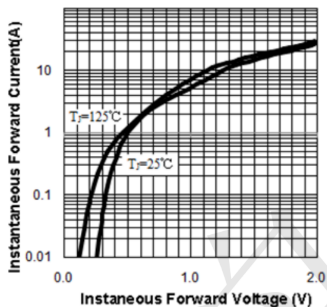
Fig.3 Typical Instantaneous Forward Characteristics
