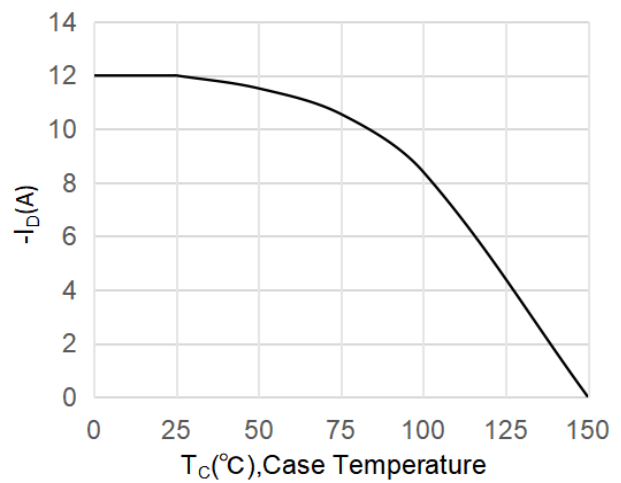
Figure 10: Maximum Continuous Drian Current vs. Ambient Temperature
