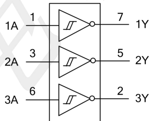
Logic symbol
