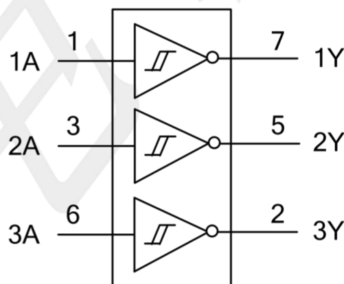
Logic symbol
