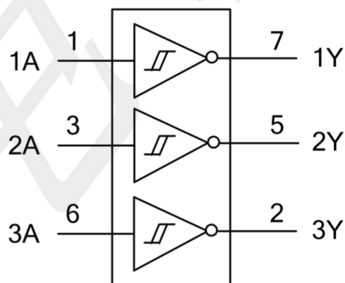
Logic symbol
