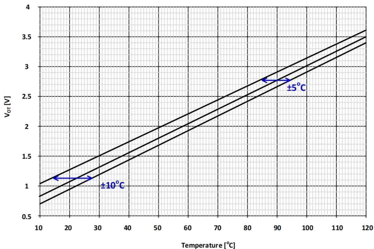
图 4: 温度- V_{OT} 特性曲线 (典型值) Figure 4. Temperature Profile of V_{OT} (Typical)
