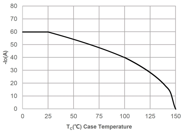
Current De-rating
