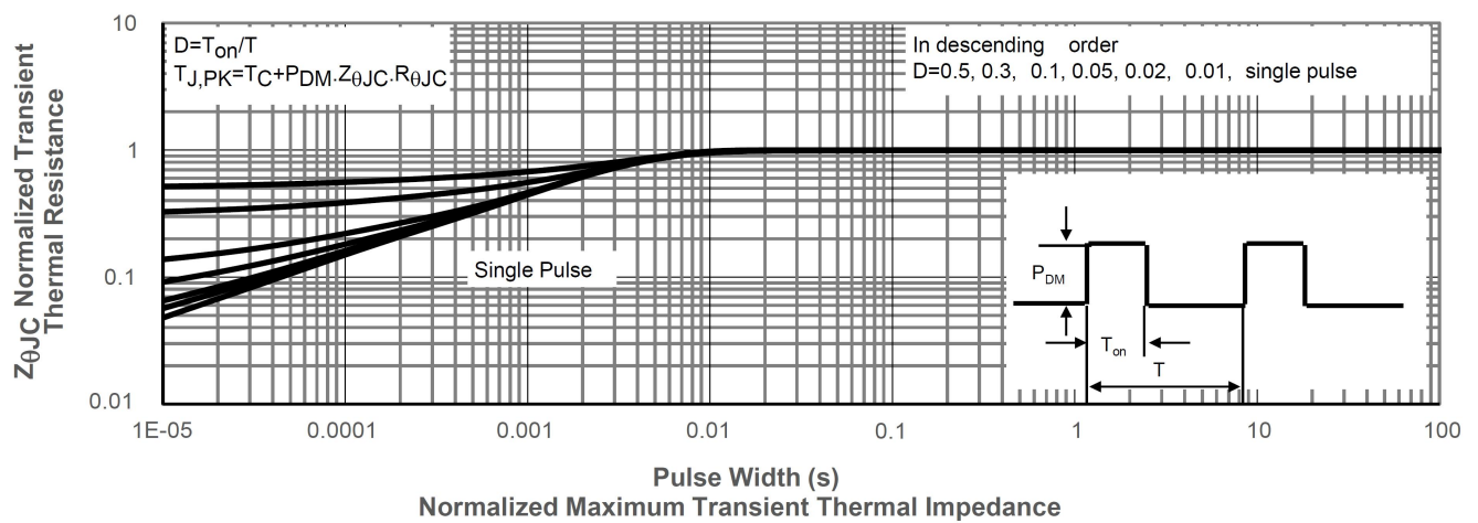
Maximum Safe Operating Area
