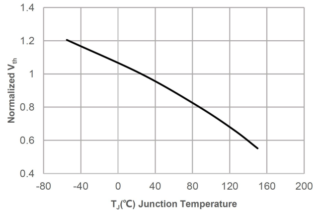
Normalized Threshold Voltage vs. Junction Temperature
