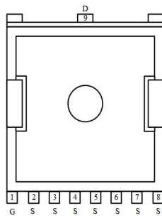
TOLL-8L
