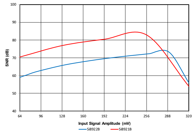
Figure 15. Si892xB Signal-to-Noise Ratio (dB) vs. Input Signal Amplitude (mV)
