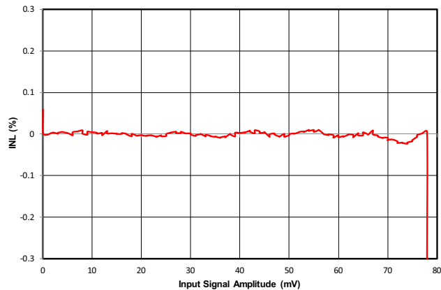
Figure 10. Si8921A Nonlinearity (%) vs. Input Signal Amplitude (mV)
