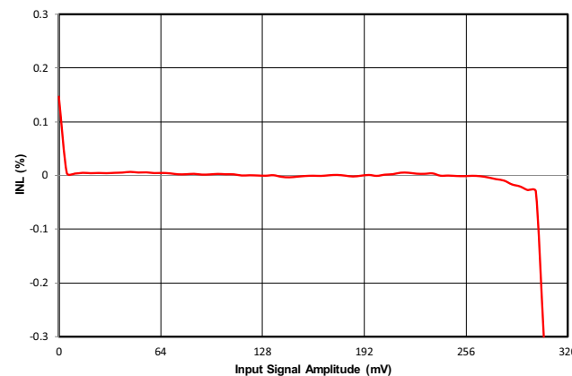
Figure 11. Si8922B Nonlinearity (%) vs. Input Signal Amplitude (mV)
