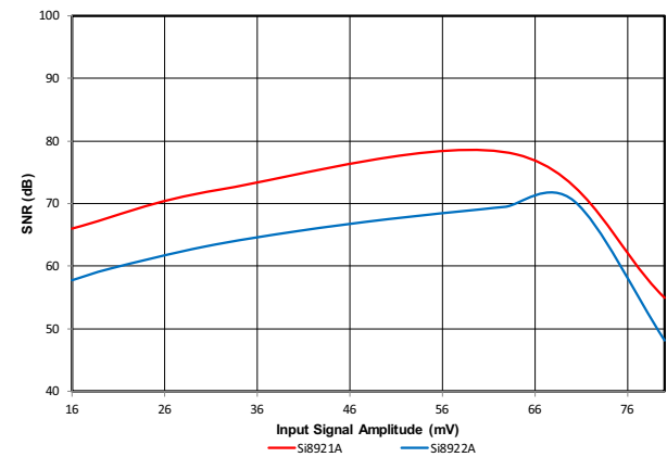
Figure 16. Si892xA Signal-to-Noise Ratio (dB) vs. Input Signal Amplitude (mV)
