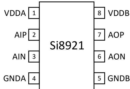
Figure 3. Si8921 Pinout (Top View)
