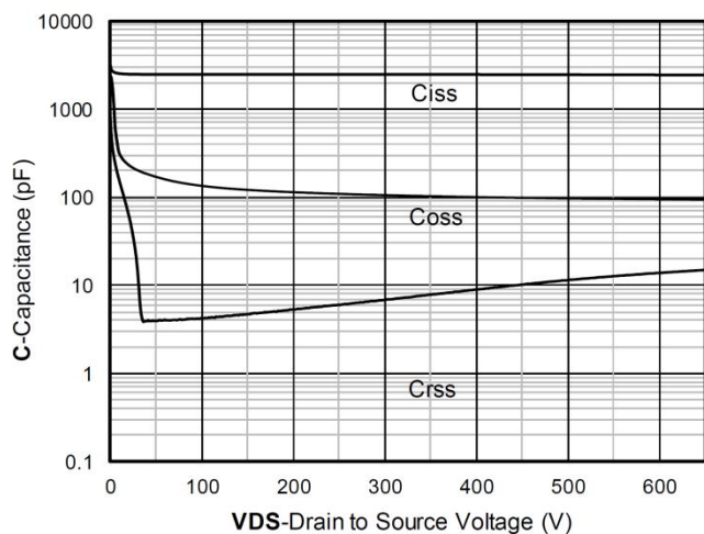
Capacitance Characteristics; typical values
