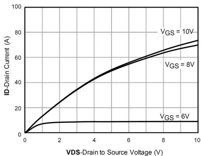
Output Characteristics; typical values
