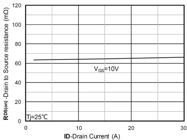
RDS(on) vs. Drain Current; typical values
