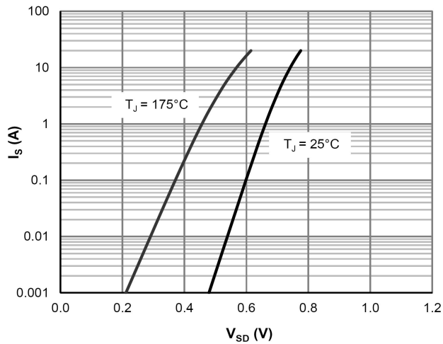
Body-Diode Characteristics
