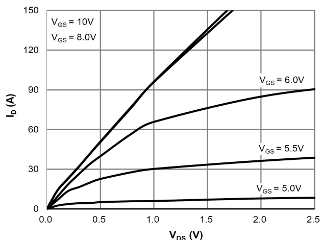
Saturation Characteristics
