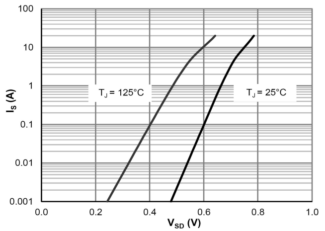
Body-Diode Characteristics
