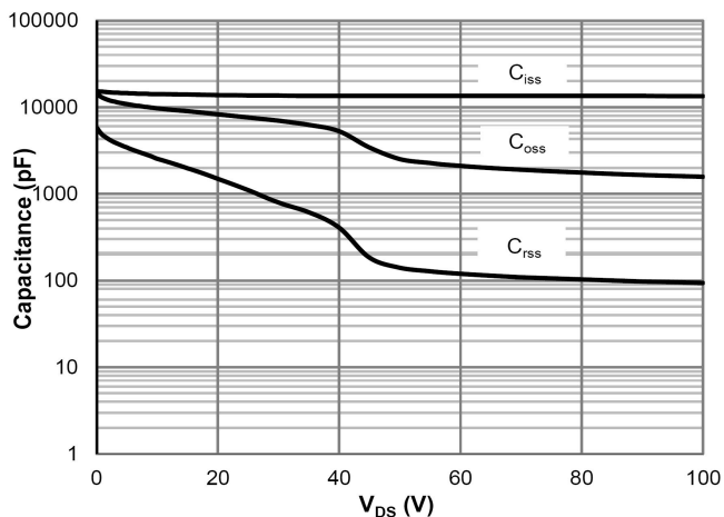
Capacitance Characteristics
