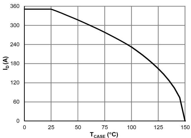
Current De-rating
