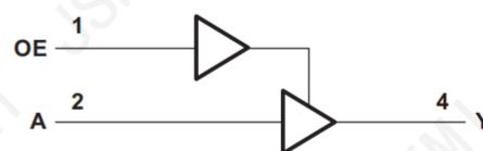
Simplified Schematic
