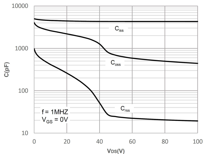
Capacitance Characteristics
