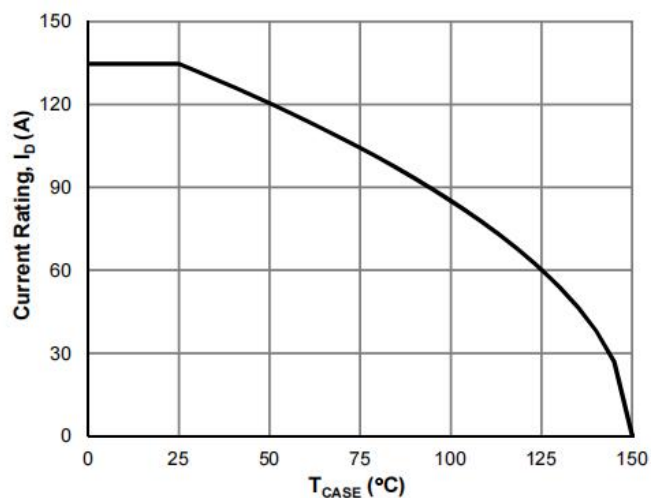
Current De-rating
