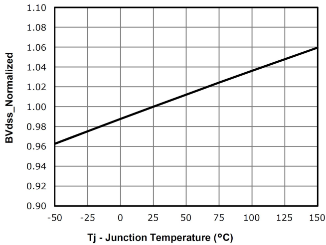
BVdss vs. Temperature
