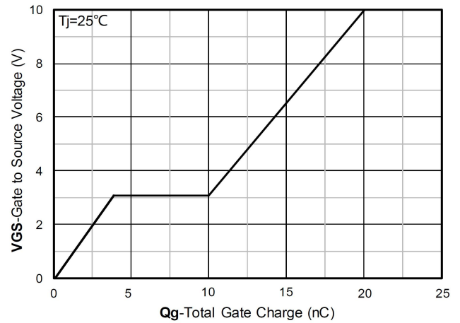
Gate Charge
