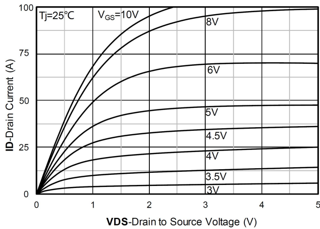
Output Characteristics
