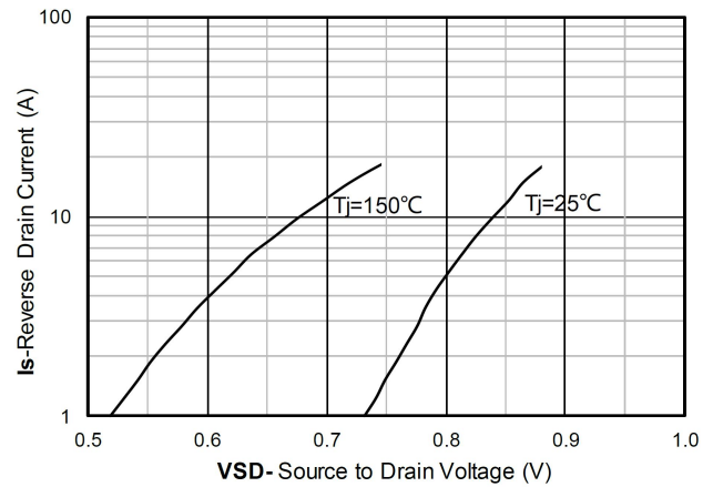
Forward characteristics of reverse diode
