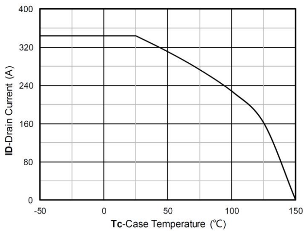
Current dissipation
