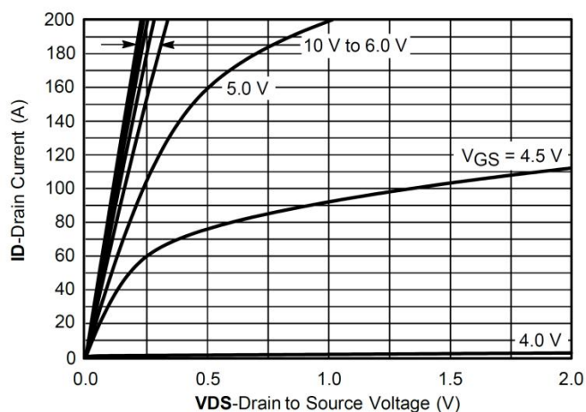
Output Characteristics
