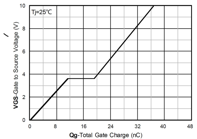
Gate Charge
