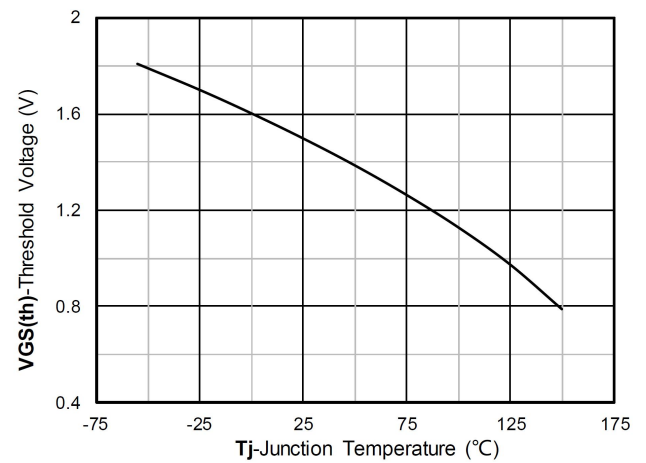
Gate Threshold voltage; typical values
