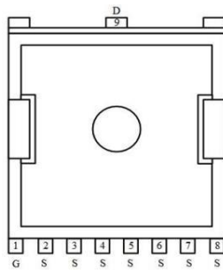
TOLL-8L
