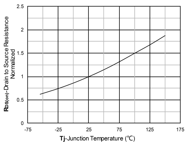
Normalized On-Resistance
