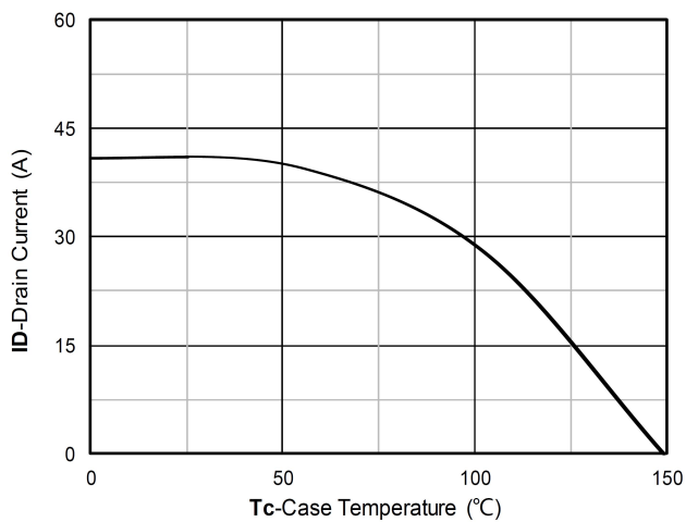
Current dissipation
