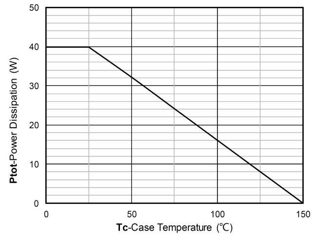
Power dissipation
