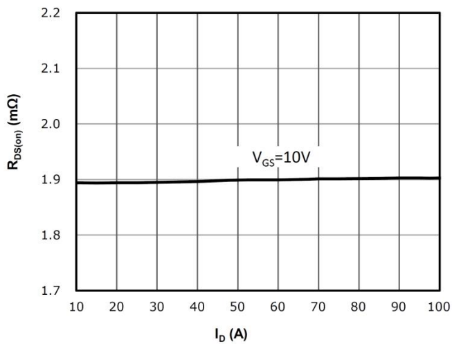
R_{DS(on)} vs Drain Current and Gate Voltage
