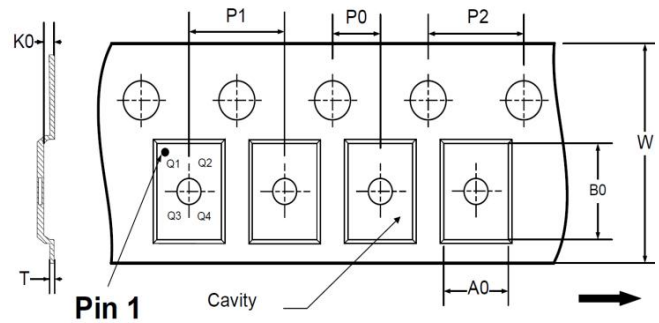
TAPE DIMENSIONS
