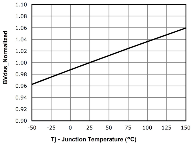
BDSS vs. Temperature
