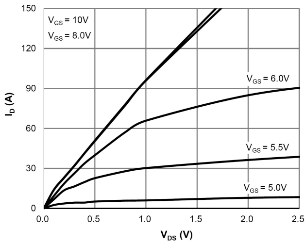
Saturation Characteristics
