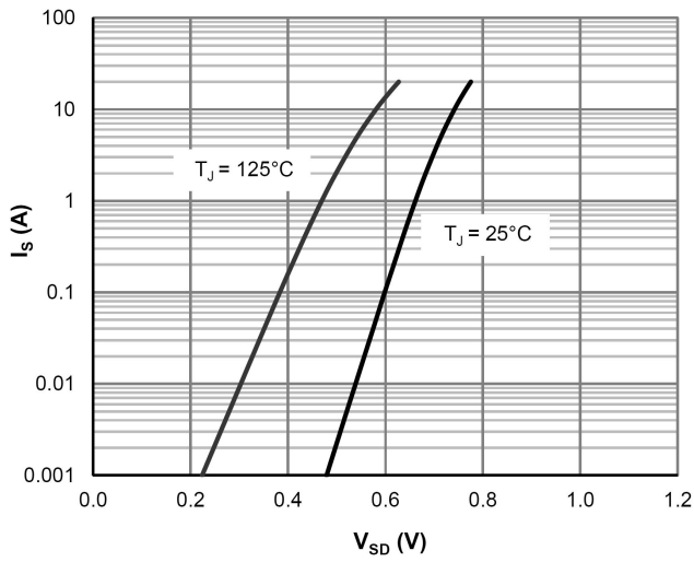
Body-Diode Characteristics
