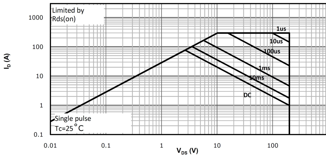
Safe Operating Area
