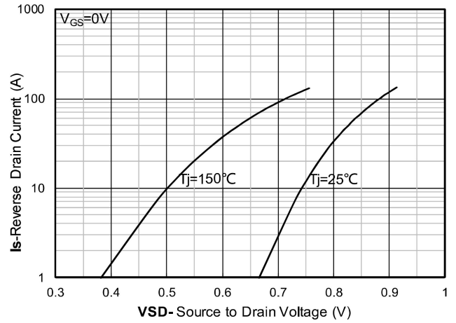
Forward characteristics of reverse diode; typical values
