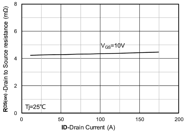
R_{DS(on)} vs. Drain Current; typical values
