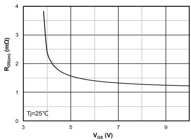
R_{DS(on)} vs Gate Voltage
