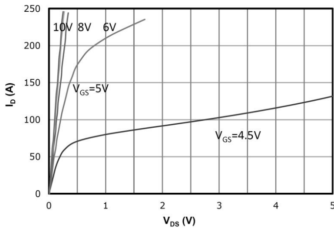
Output Characteristics
