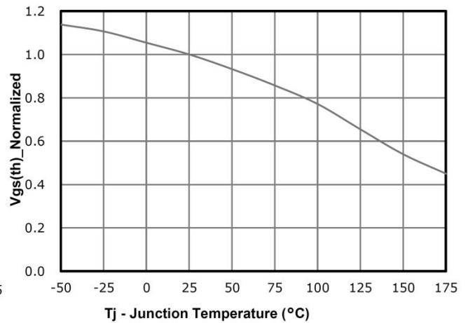
V_{GS(th)} vs. Temperature
