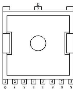
TOLL-8L
