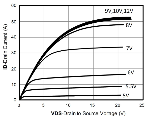
Output Characteristics; typical values
